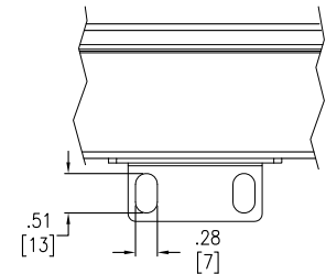
VIEW E (MOUNTING BRACKET-ENLARGED)
