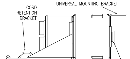
VIEW F (RIGHT SIDE VIEW-ENLARGED)
