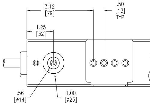
VIEW B (ENLARGED)
