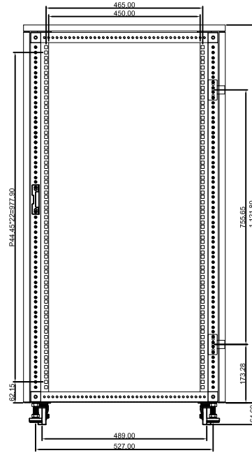
Front view Without Front Door
