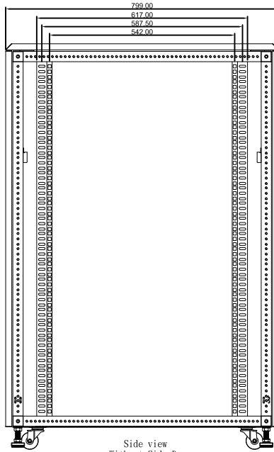
Side view Without Side Door
