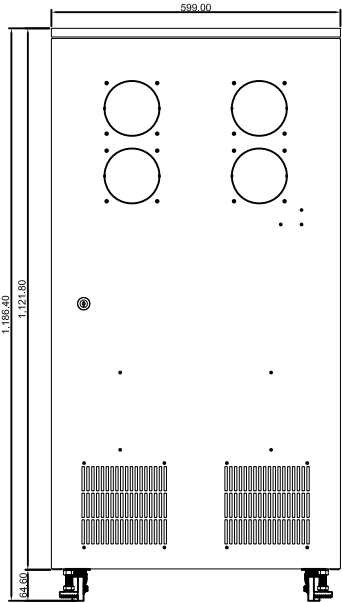
Rear view
