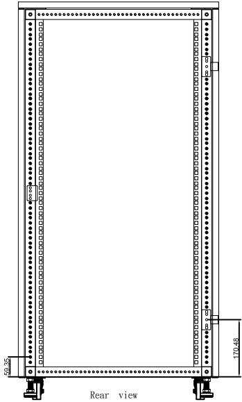
Rear view Without Rear Door
