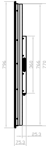
Left-side View
