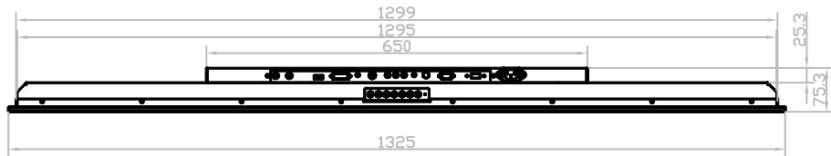
Bottom View
