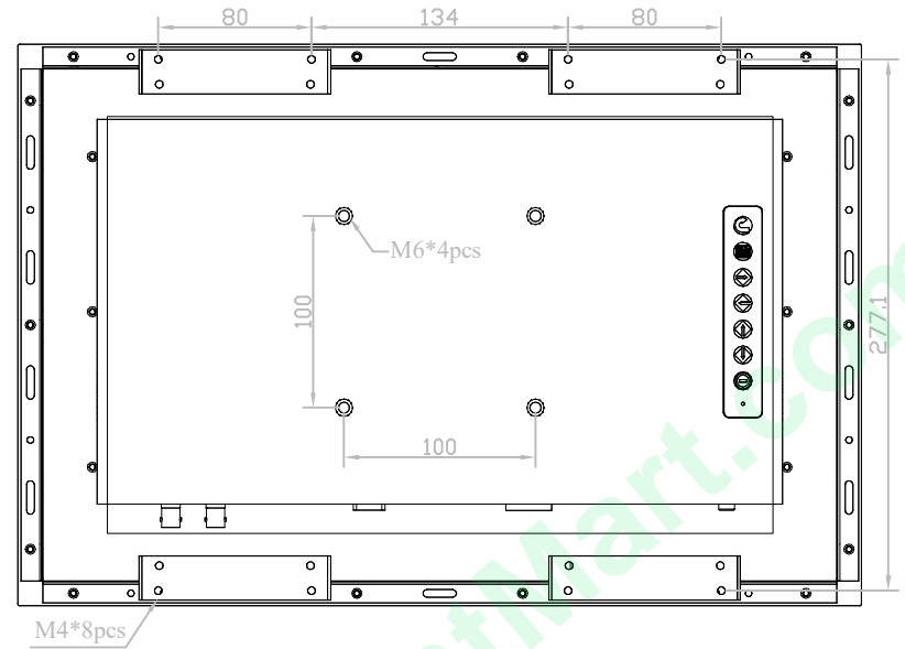
Rear View
