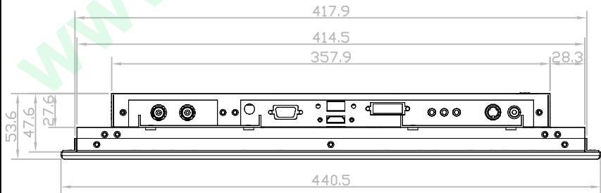
Bottom View
