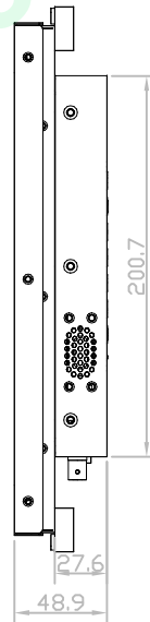
Left-side View
