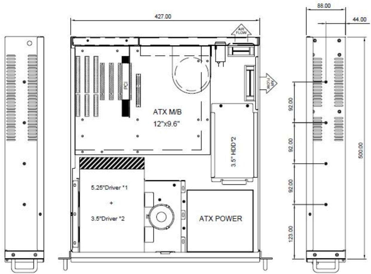
Left-side View
