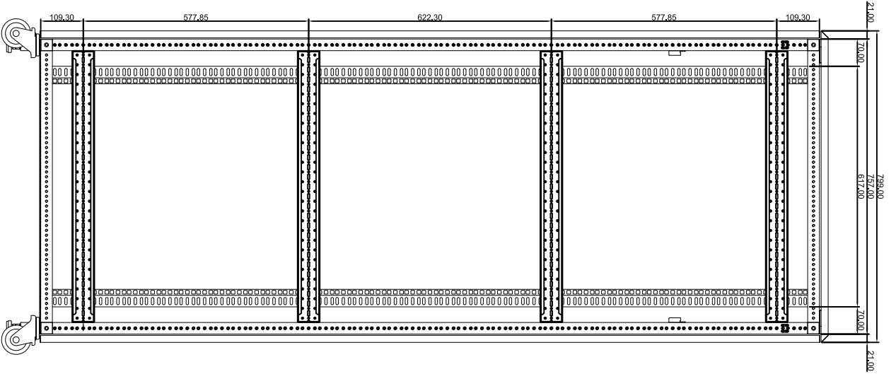
Side view Without Side Door
