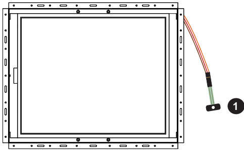
① DA Light sensor on ID-19P ( 66cm from AD board to sensor end )
