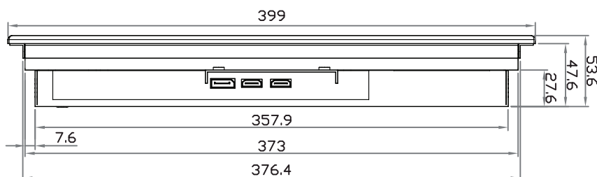
Bottom View
