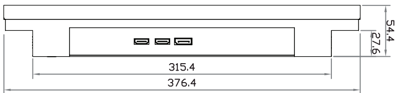
Bottom View
