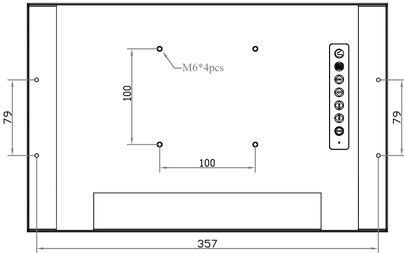
Rear View
