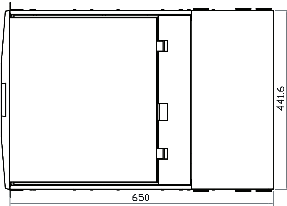
Top View
