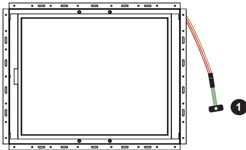
① DA Light sensor on ID-19Pw model ( 66cm from AD board to sensor end )
