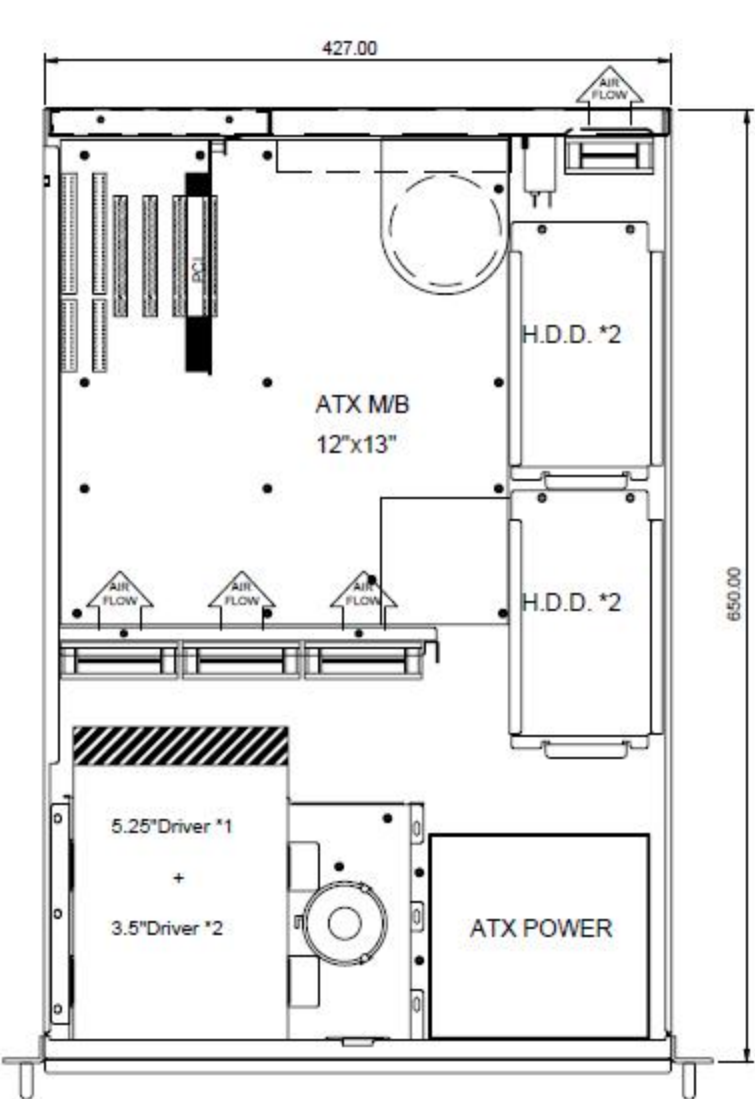
Top View
