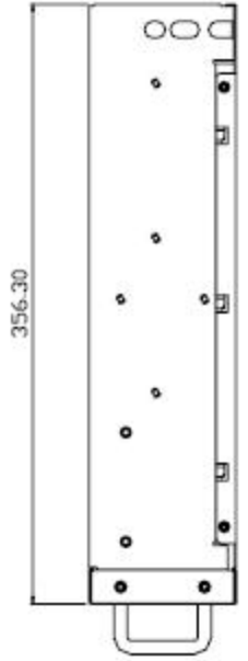
Left-side View
