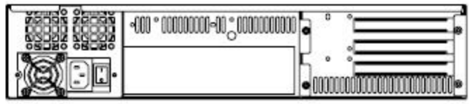
Rear View(GHI-252H)
