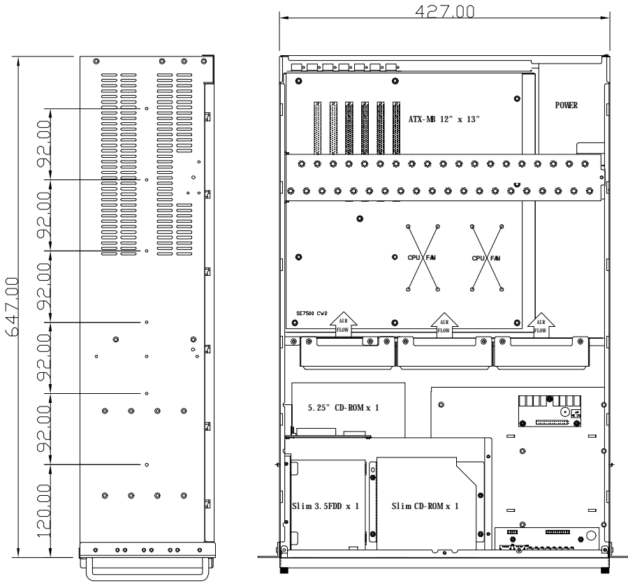
Left View
