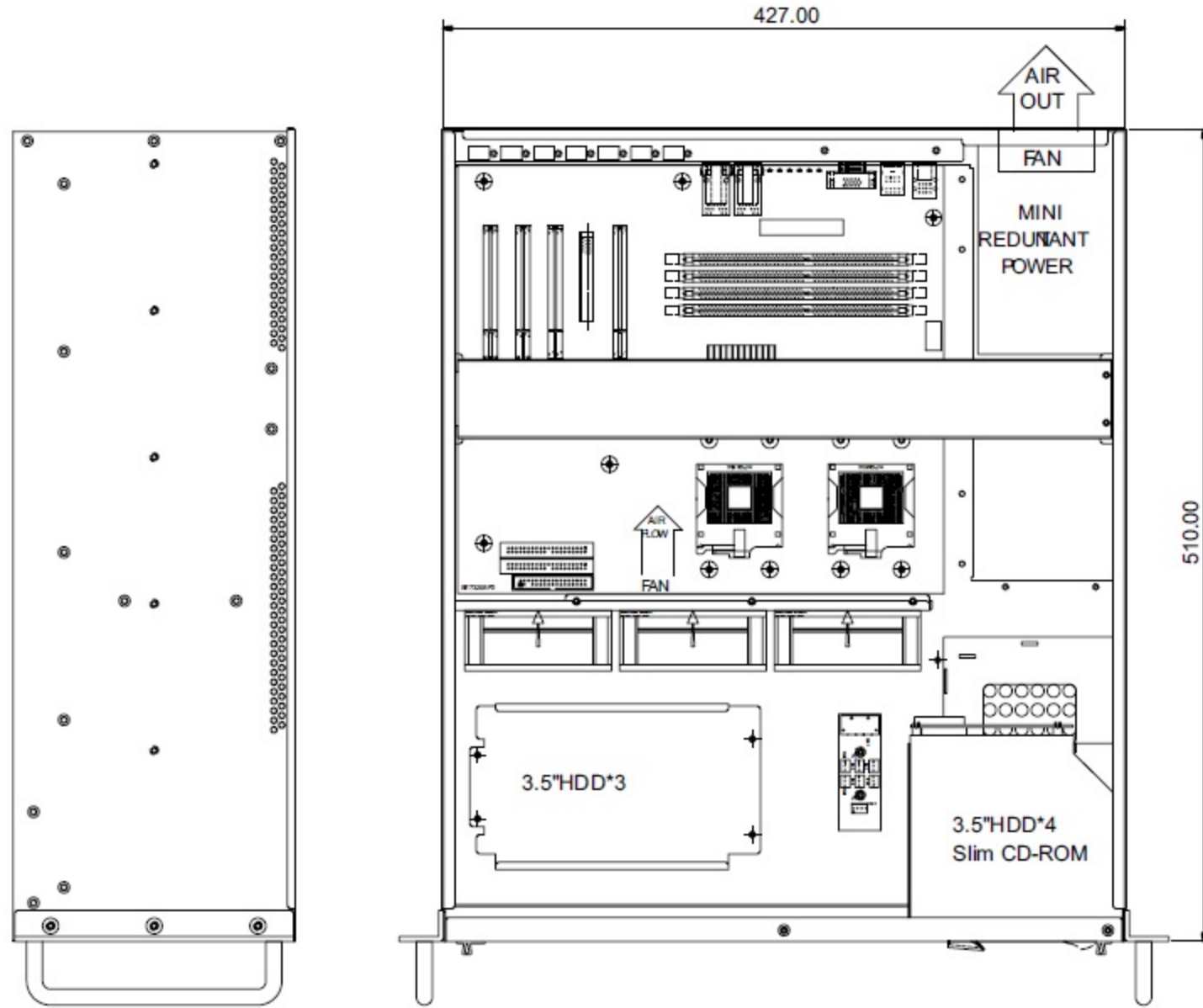
Left-side View
