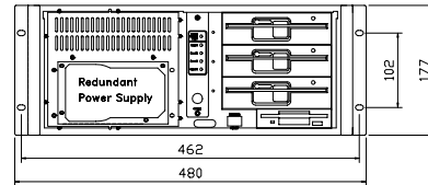
Front in-side view
