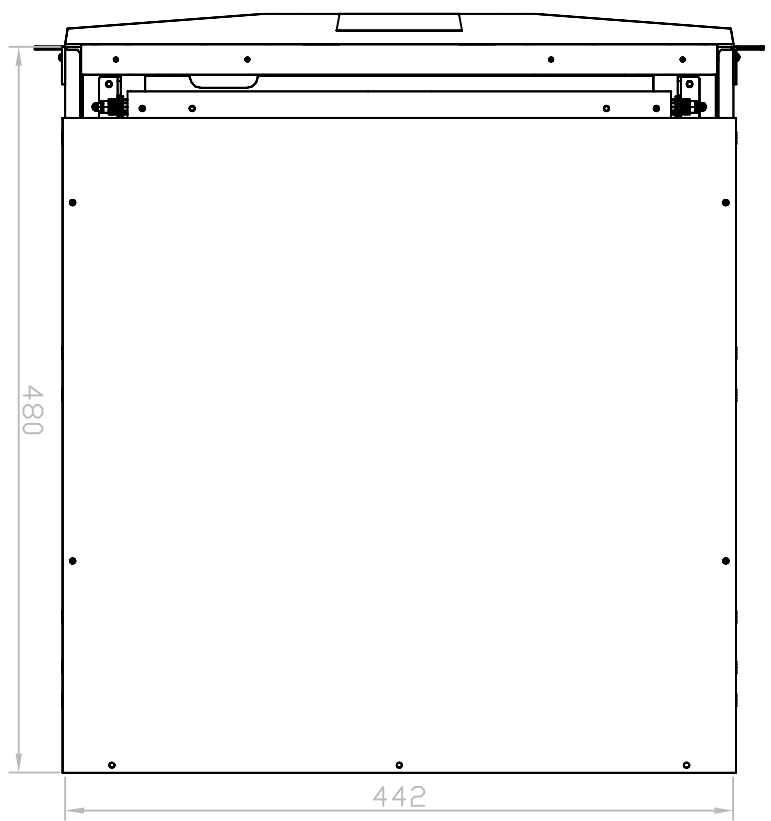
Top View
