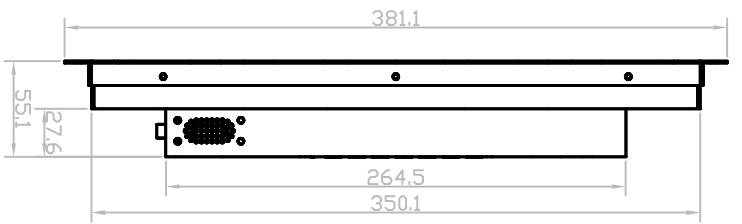
Left-side View
