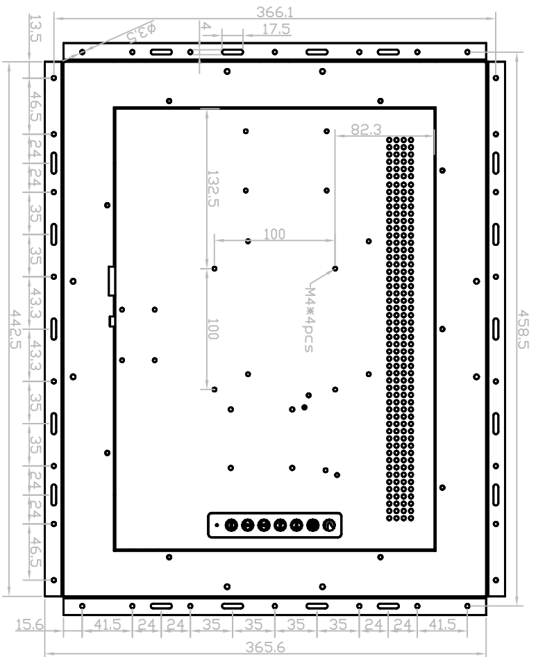
Rear View
