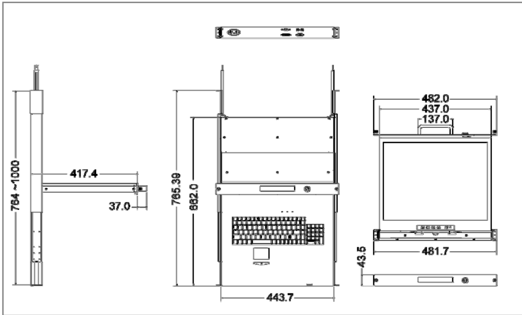
Figure 1-1. 20.1" LCD Console Dimension
