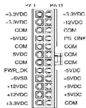
Main Power Connector
