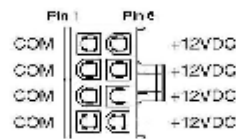
+12V 8P Power Connector
