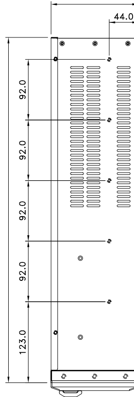
Right-side View
