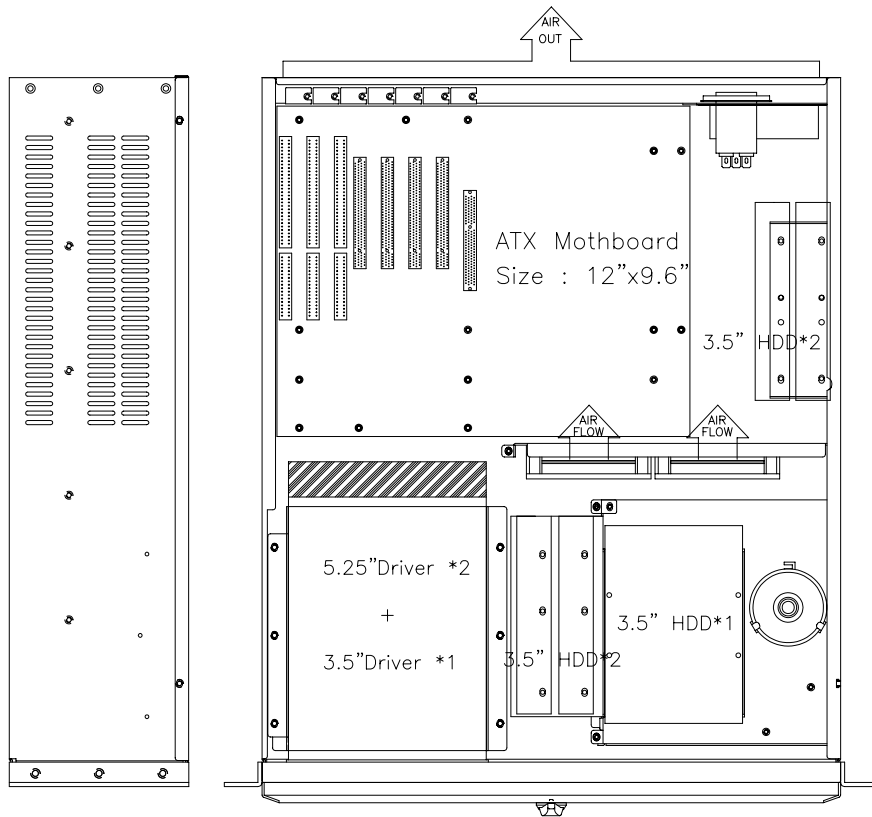
Left-side View
