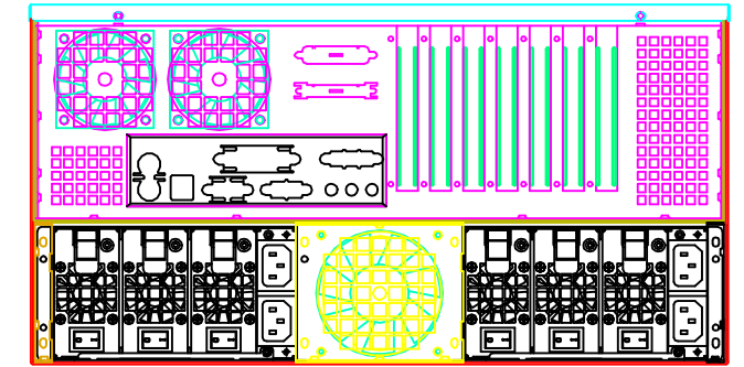
Rear View
