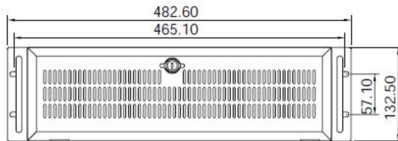
Front in-side view
