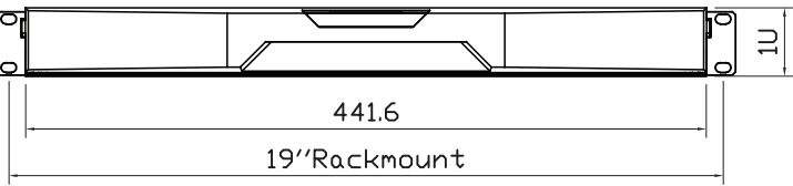
Front View
