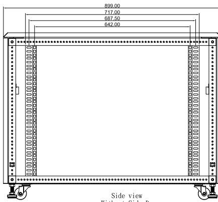
Side view Without Side Door
