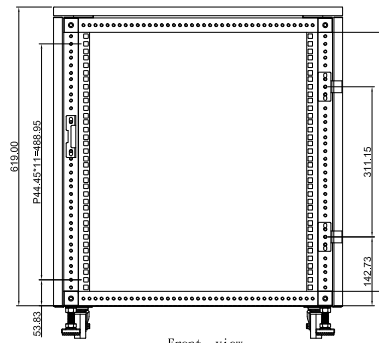
Front view Without Front Door
