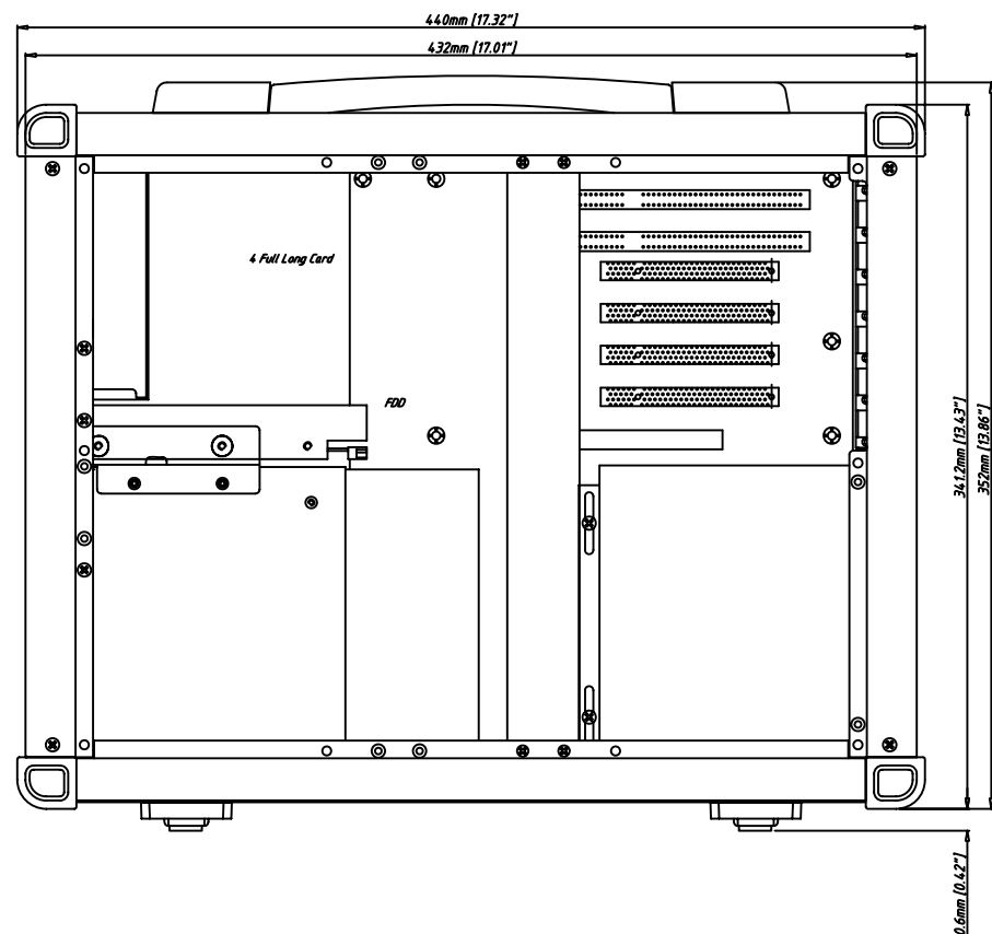
Front View
