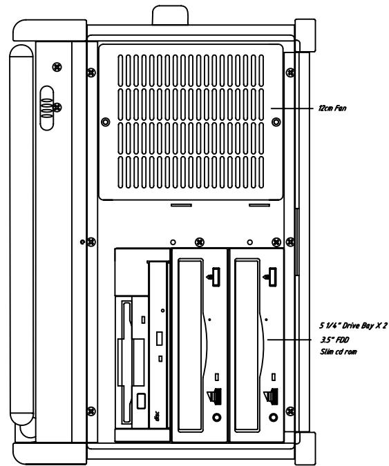
Right Side
