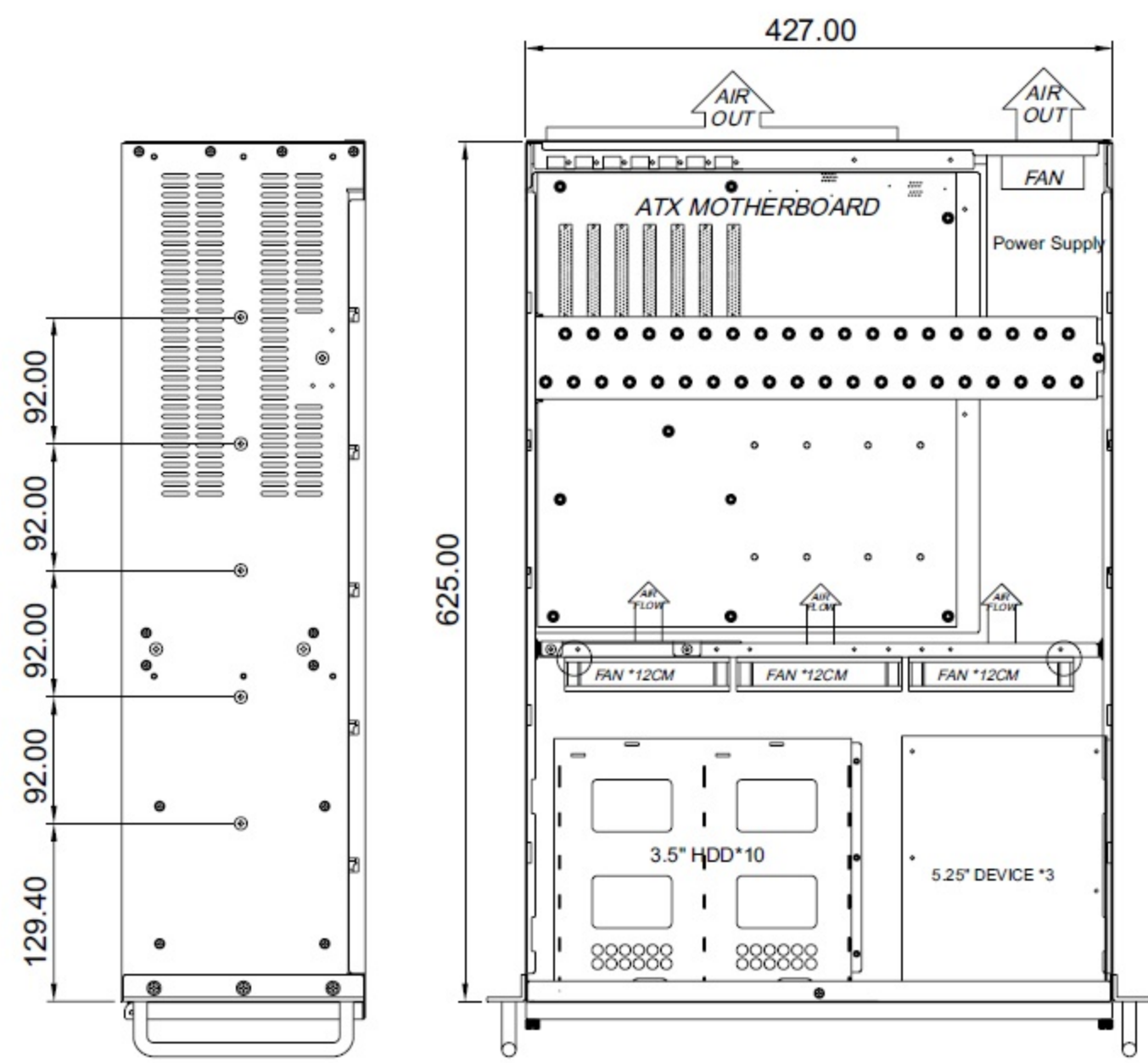
Top View
